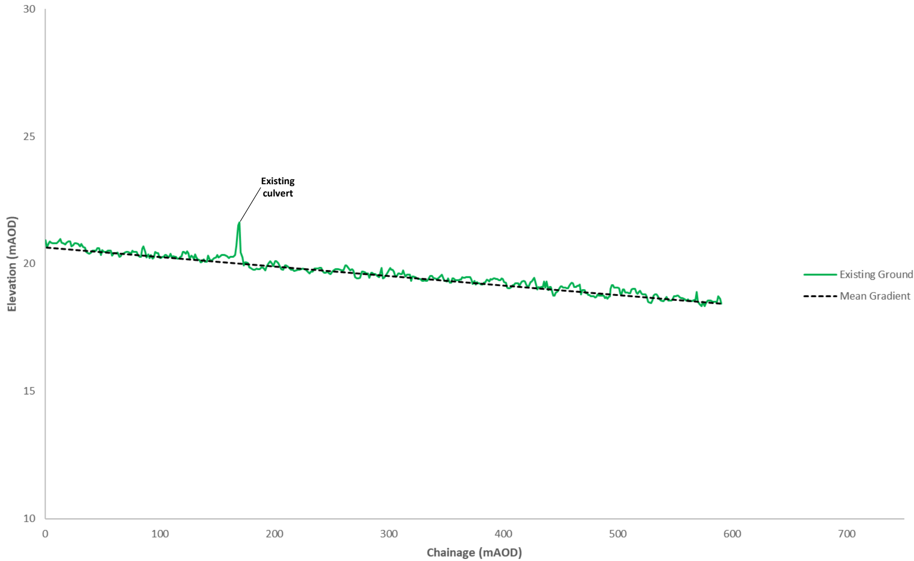
Existing Long Section
