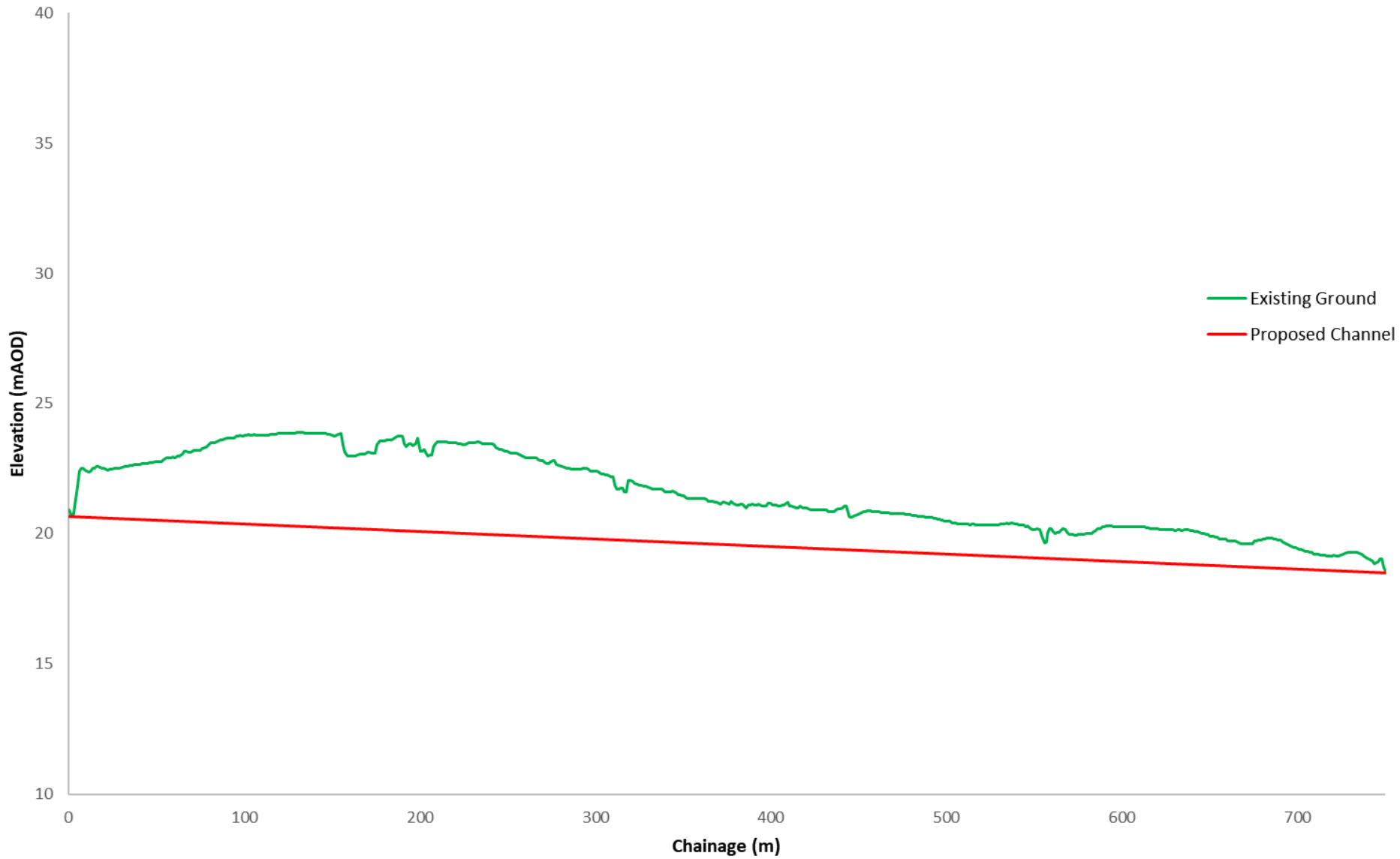
Proposed Long Section (indicative)
