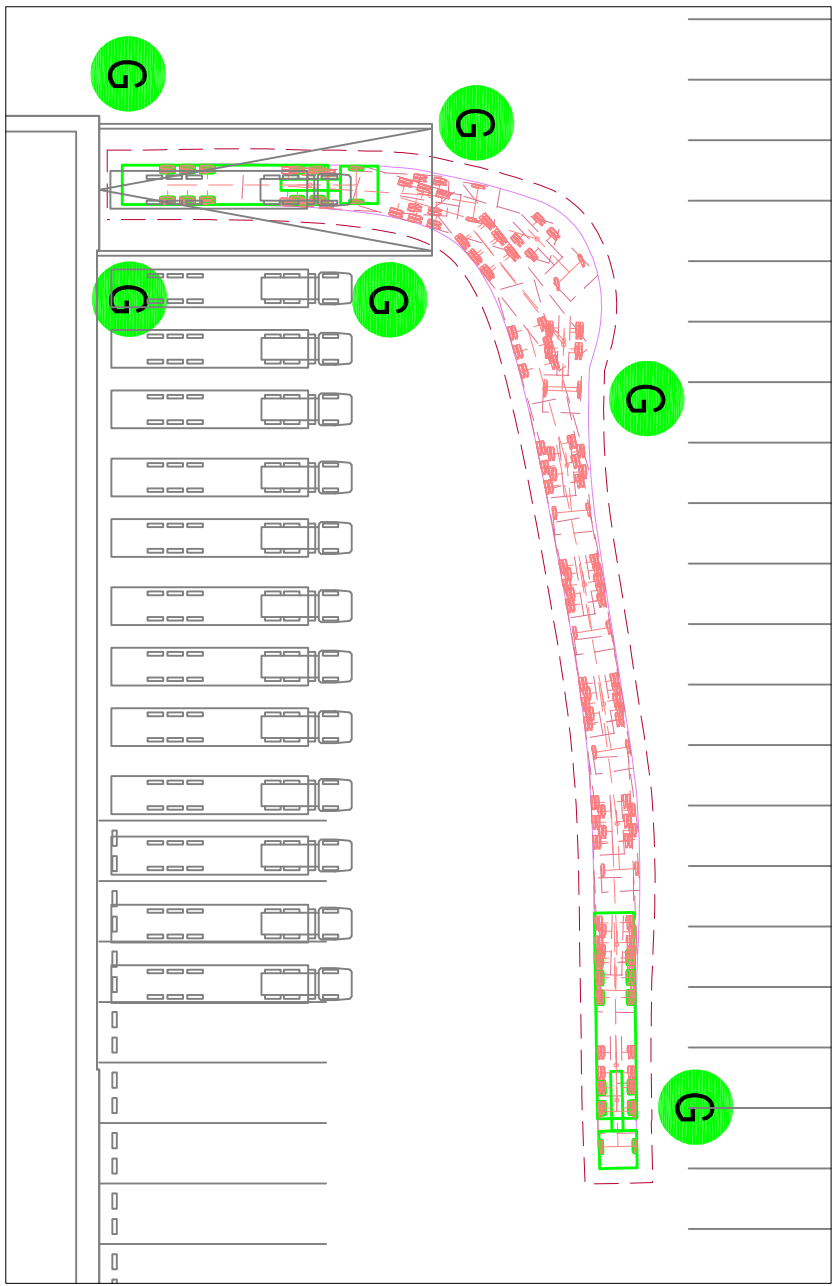
LARGE 'HGV' VEHICLE FORWARD MANOEUVRE FROM LEVEL ACCESS
