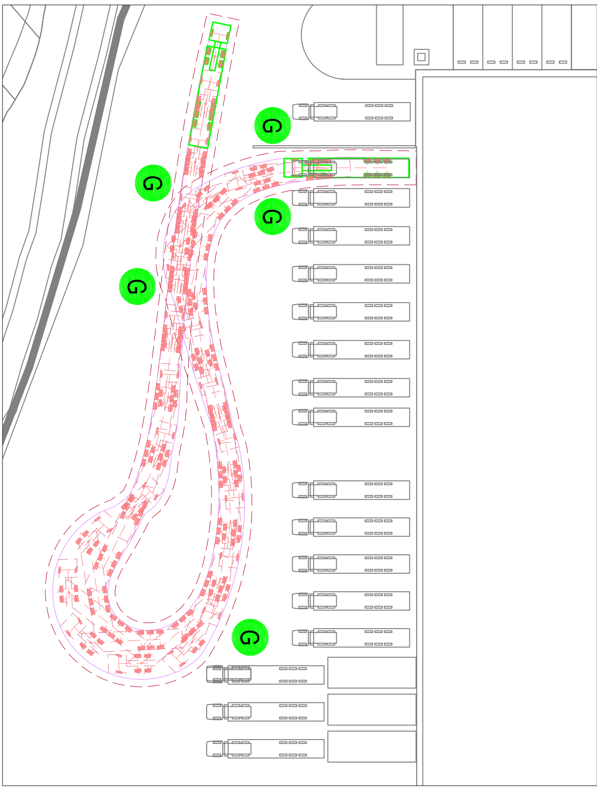
LARGE 'HGV' VEHICLE REVERSE MANOEUVRE INTO PARKING BAY
