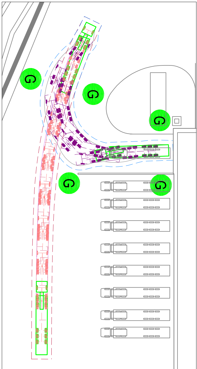
LARGE 'HGV' VEHICLE REVERSE MANOEUVRE INTO PARKING BAY
