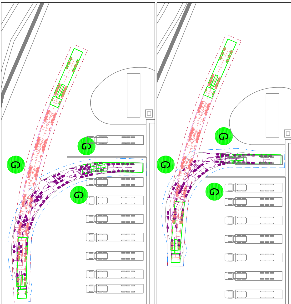
LARGE 'HGV' VEHICLE FORWARD MANOEUVRE ENTERING DISTRIBUTION CENTRE SITE & REVERSE MANOEUVRE INTO PARKING BAY
