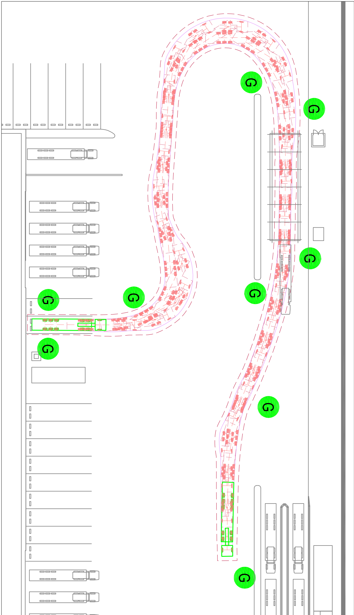
LARGE 'HGV' VEHICLE FORWARD MANOEUVRE FROM PARKING BAY
