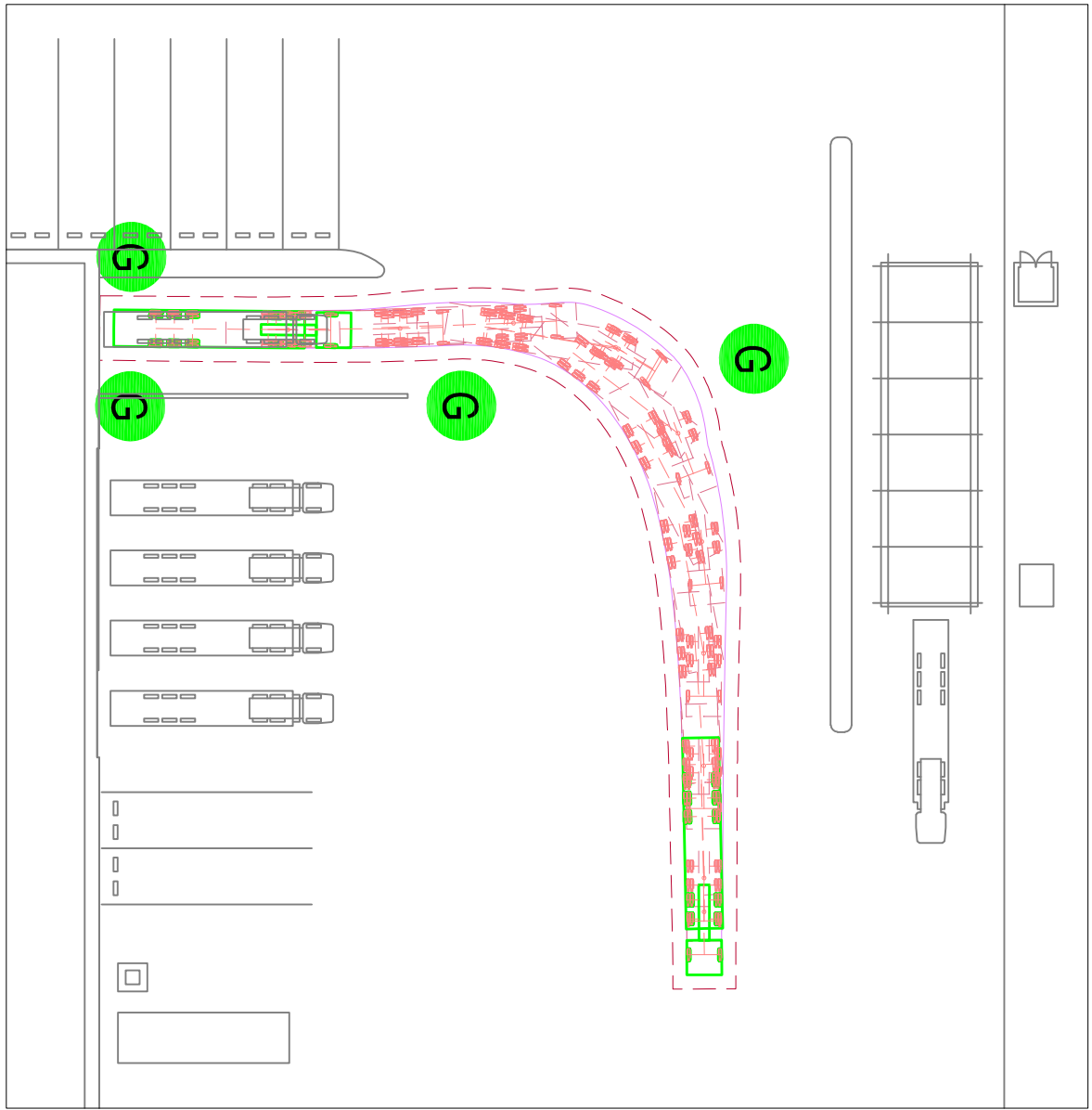
LARGE 'HGV' VEHICLE FORWARD MANOEUVRE FROM PARKING BAY
